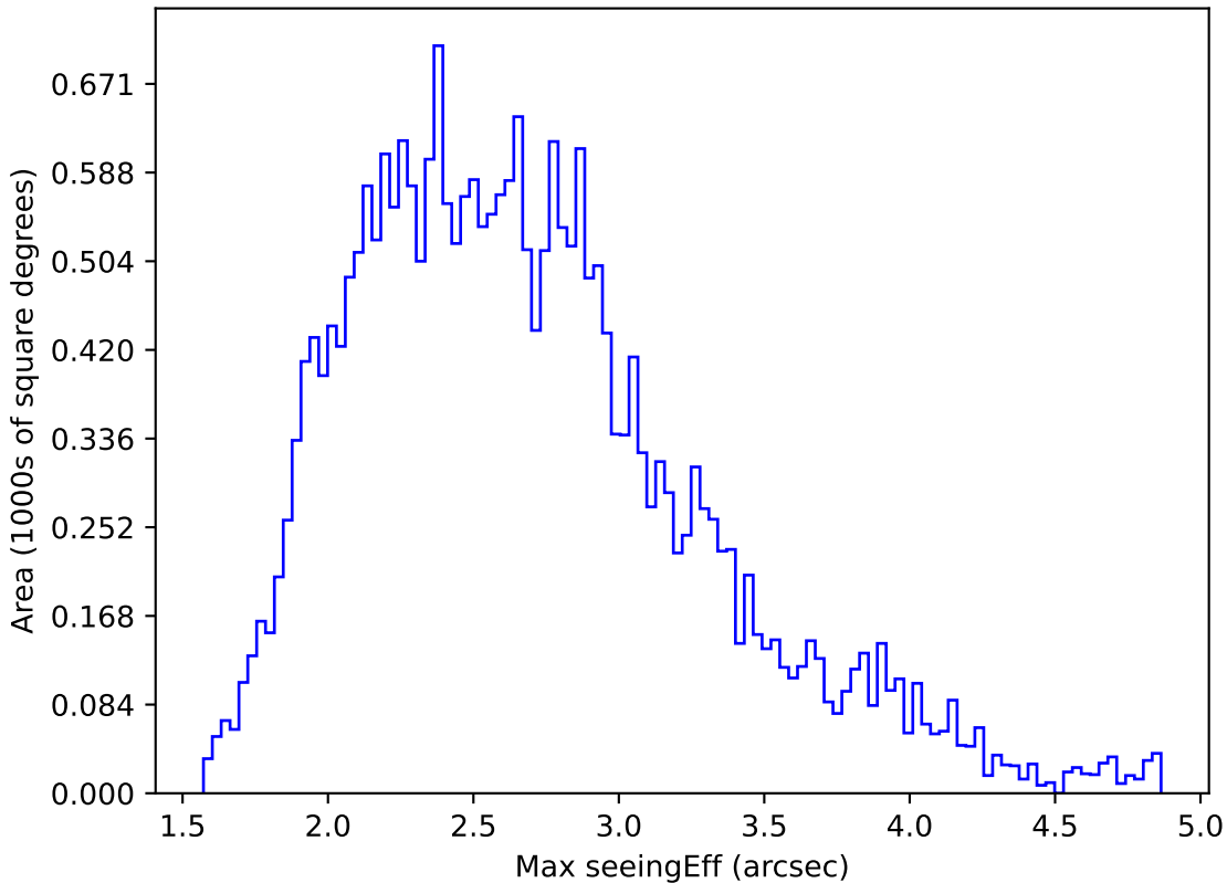
roll_pause_mjdp180_v3.4_10yrs All sky r band: Max seeingEff
