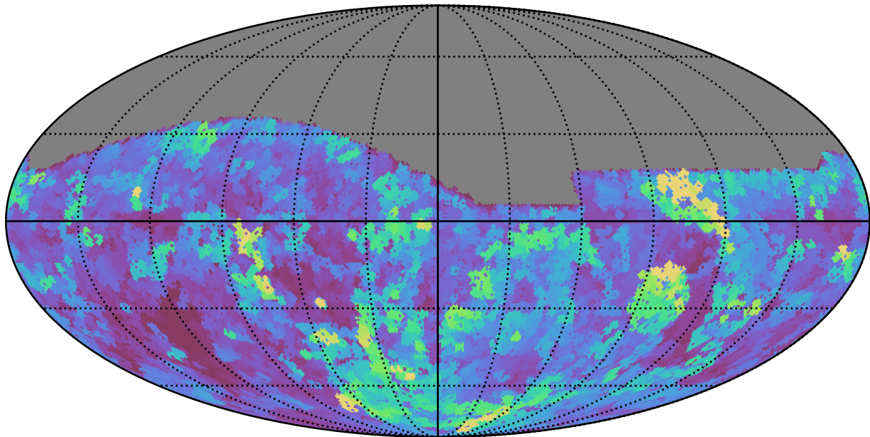
roll_pause_mjdp180_v3.4_10yrs All sky g band: Max seeingEff
