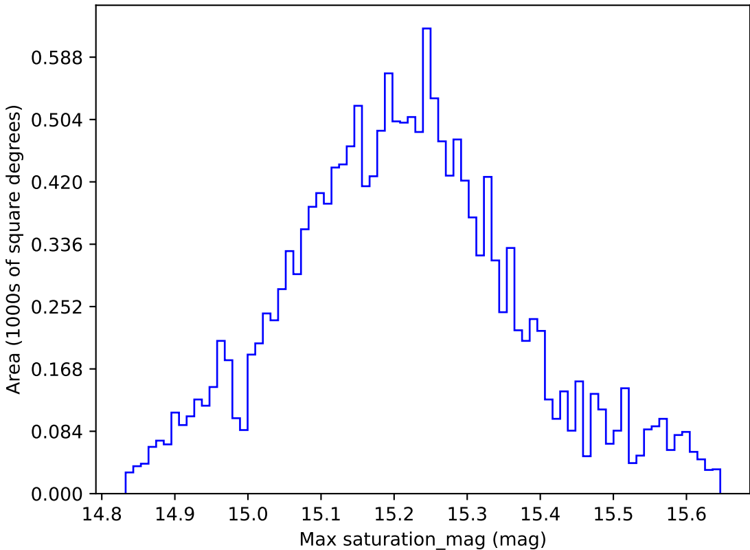
roll_pause_mjdp180_v3.4_10yrs WFD z band: Max saturation_mag
