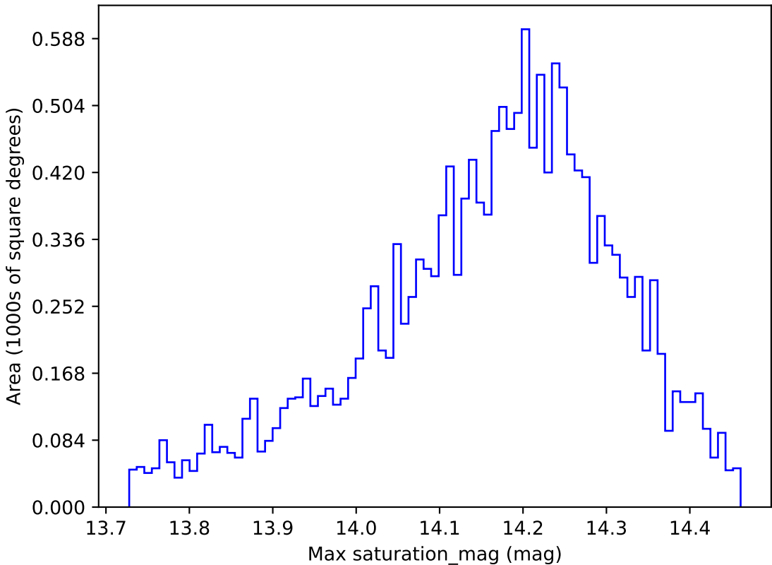
roll_pause_mjdp180_v3.4_10yrs WFD y band: Max saturation_mag
