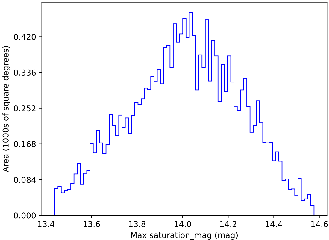
roll_pause_mjdp180_v3.4_10yrs WFD u band: Max saturation_mag
