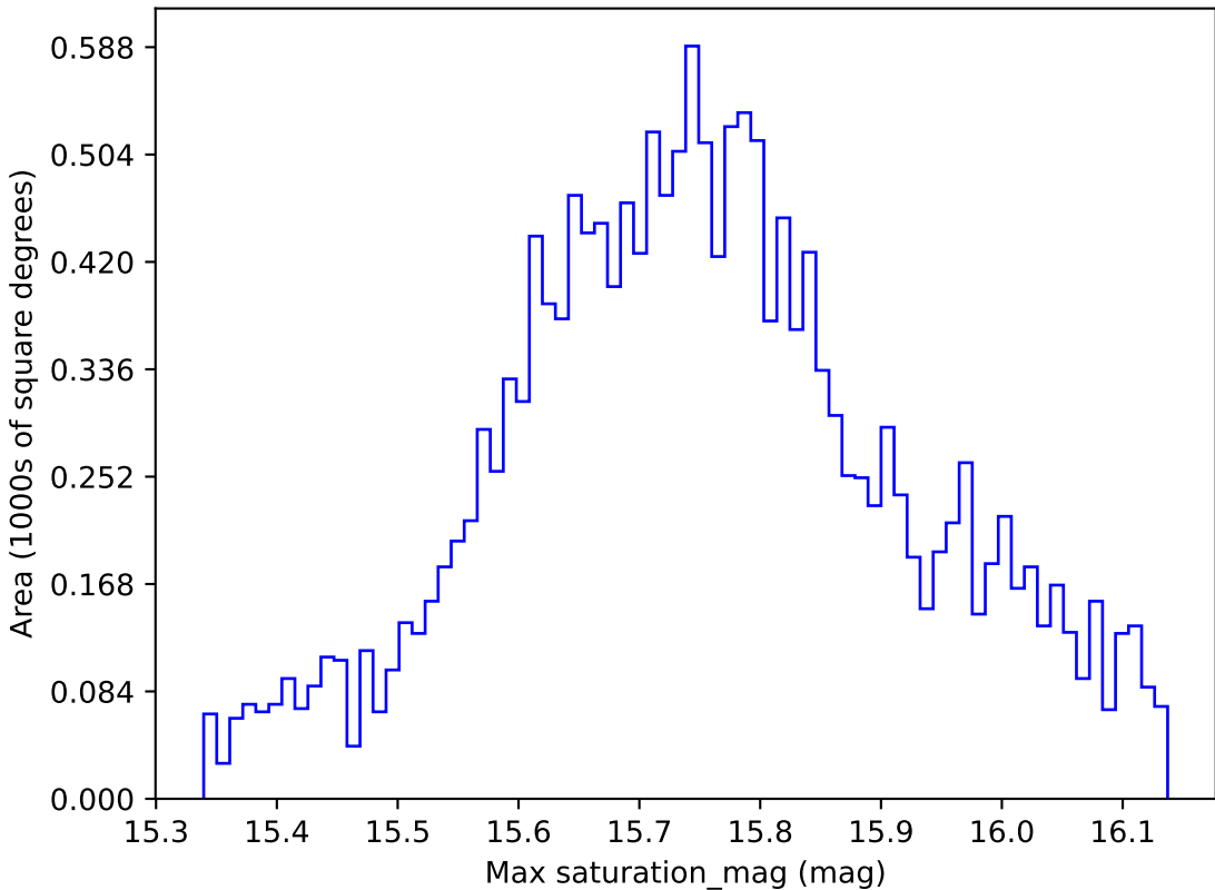
roll_pause_mjdp180_v3.4_10yrs WFD r band: Max saturation_mag
