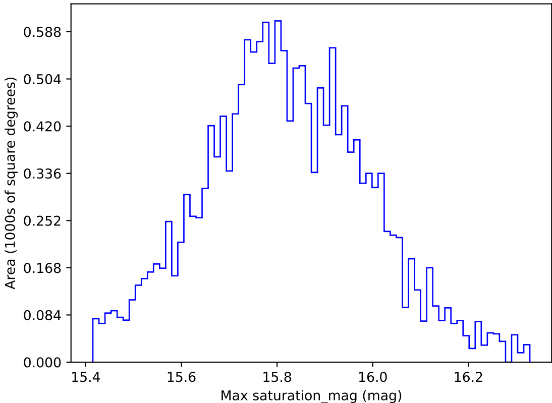
roll_pause_mjdp180_v3.4_10yrs WFD all bands: Max saturation_mag
