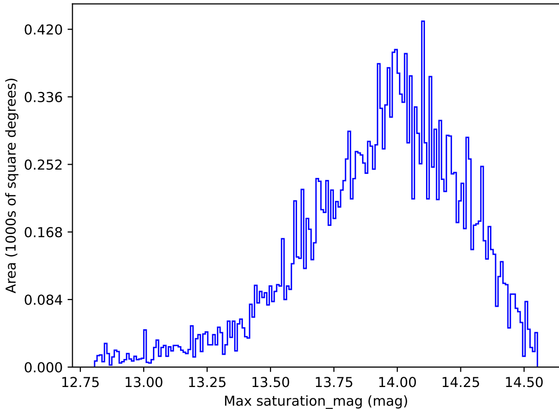
roll_pause_mjdp180_v3.4_10yrs All sky u band: Max saturation_mag
