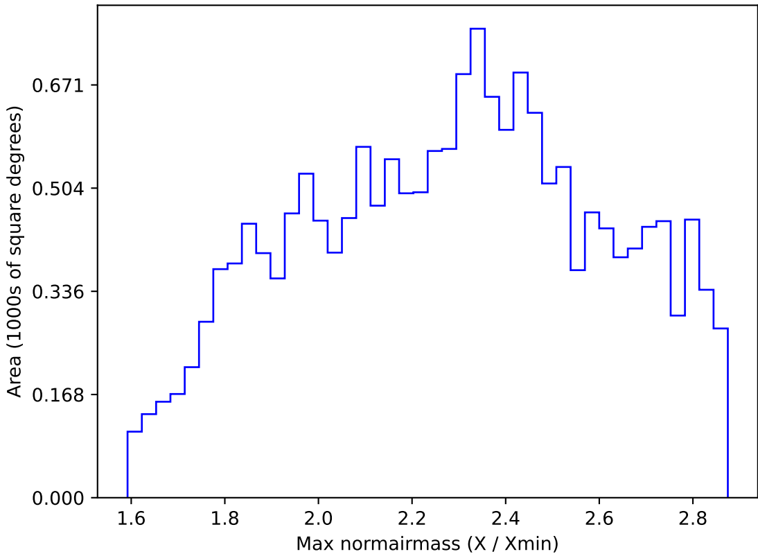
roll_pause_mjdp180_v3.4_10yrs WFD z band: Max normairmass
