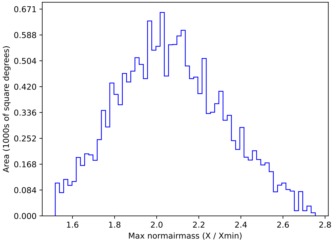
roll_pause_mjdp180_v3.4_10yrs WFD y band: Max normairmass
