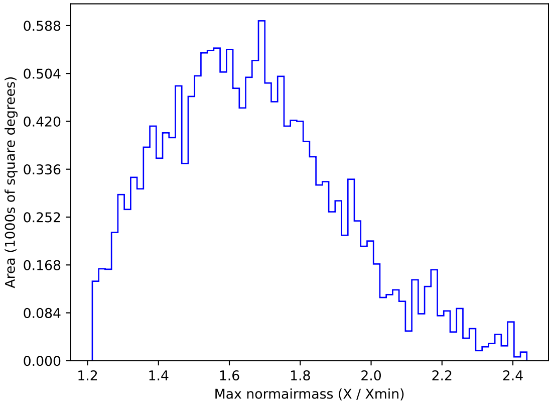
roll_pause_mjdp180_v3.4_10yrs WFD u band: Max normairmass
