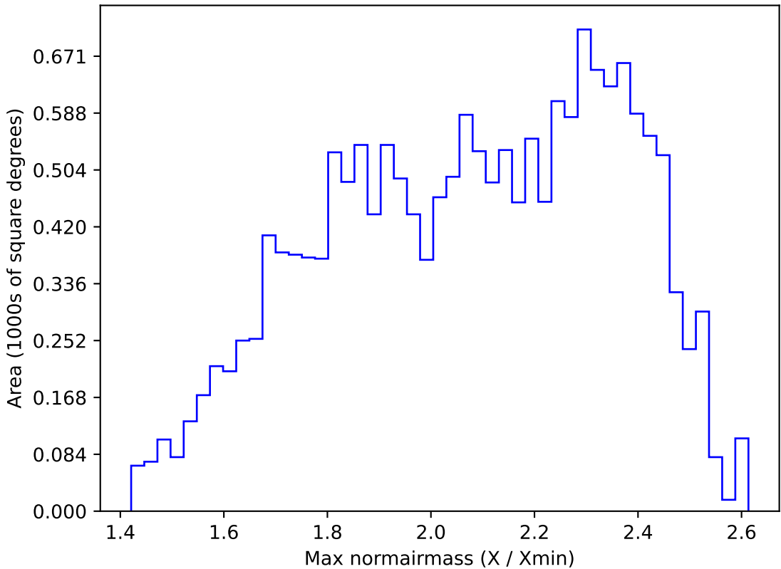
roll_pause_mjdp180_v3.4_10yrs WFD r band: Max normairmass
