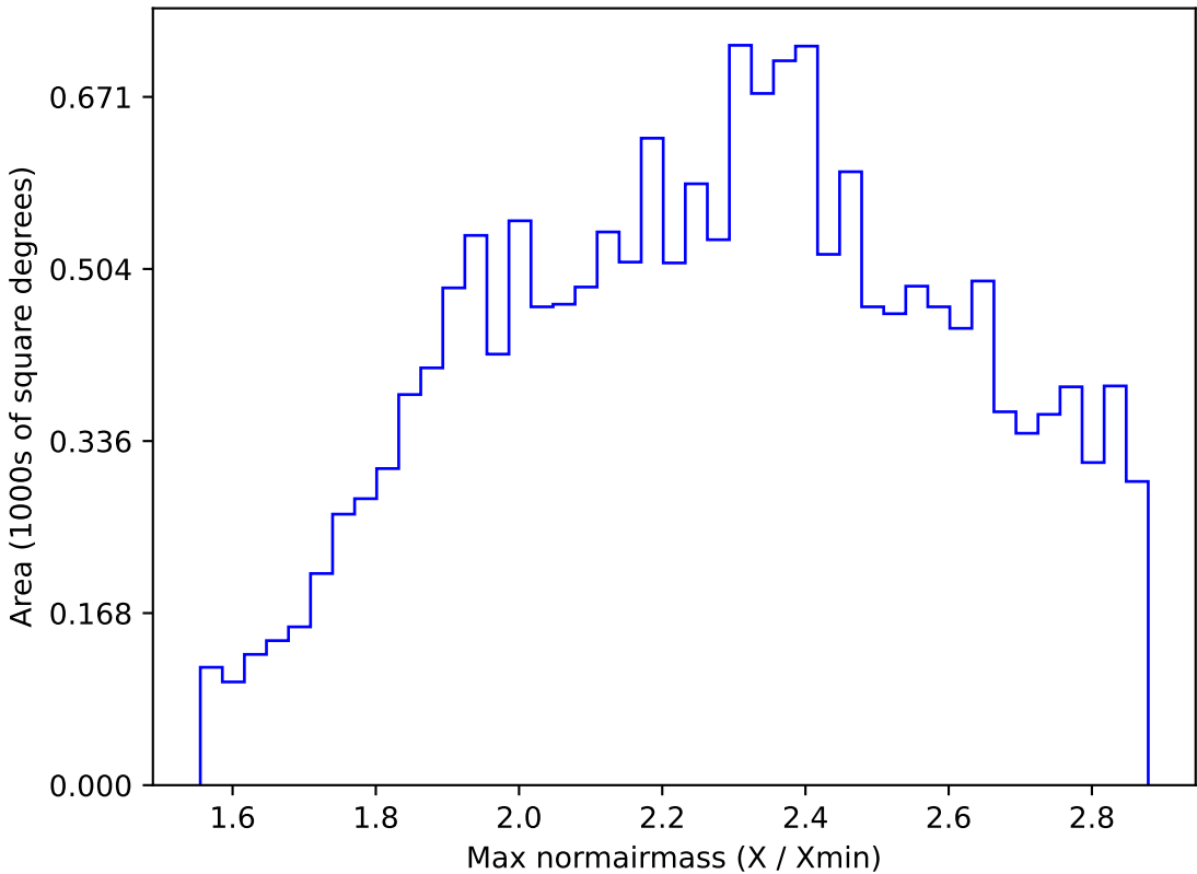
roll_pause_mjdp180_v3.4_10yrs WFD i band: Max normairmass
