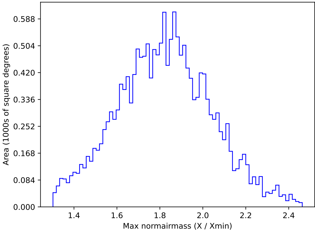
roll_pause_mjdp180_v3.4_10yrs WFD g band: Max normairmass
