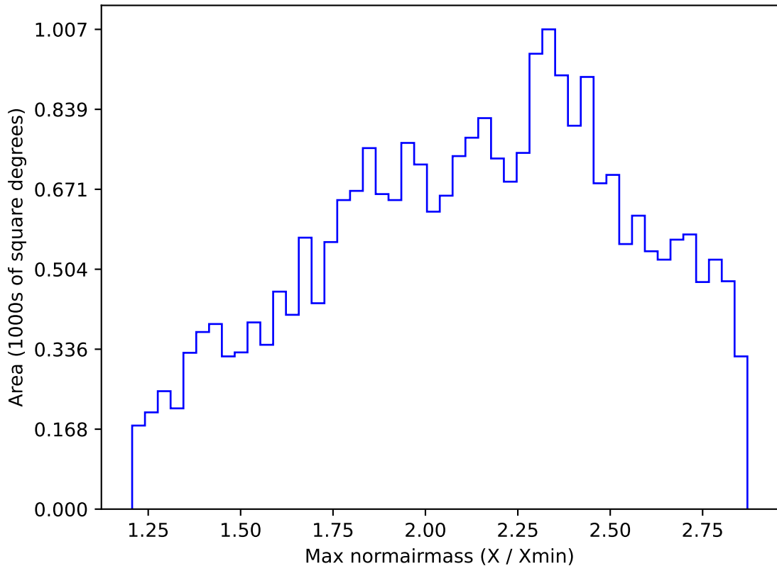
roll_pause_mjdp180_v3.4_10yrs All sky z band: Max normairmass
