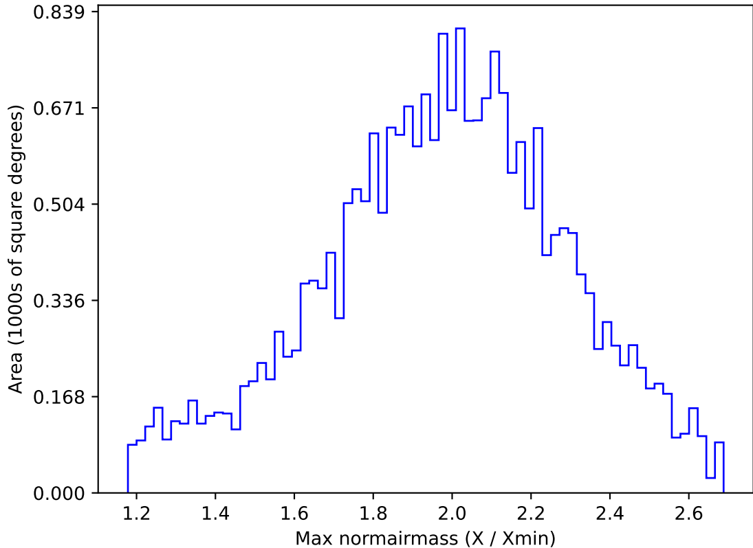
roll_pause_mjdp180_v3.4_10yrs All sky y band: Max normairmass
