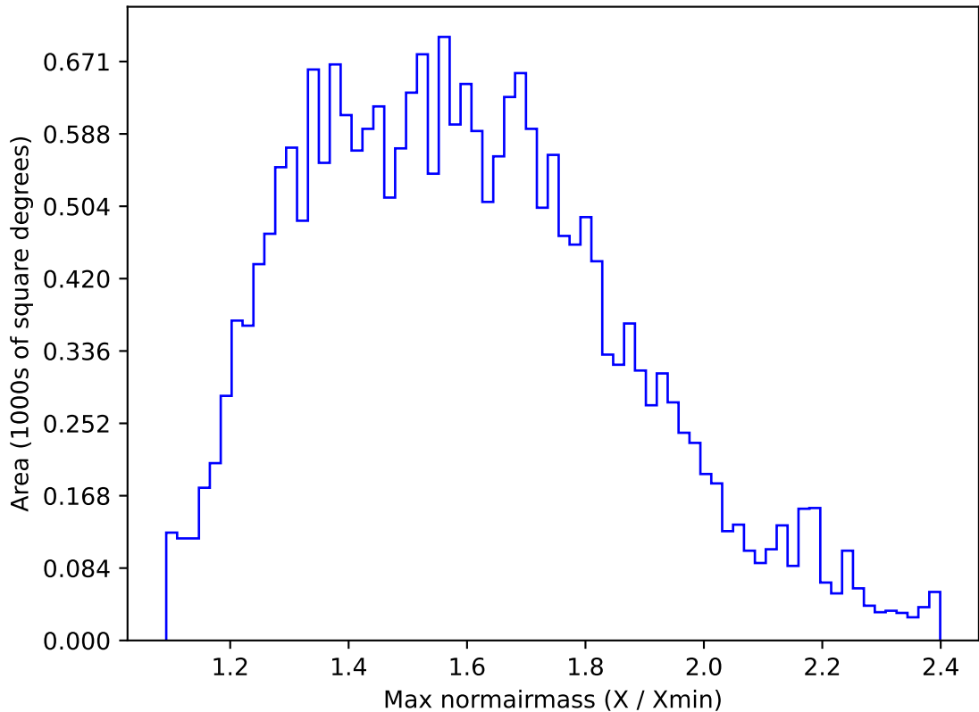
roll_pause_mjdp180_v3.4_10yrs All sky u band: Max normairmass
