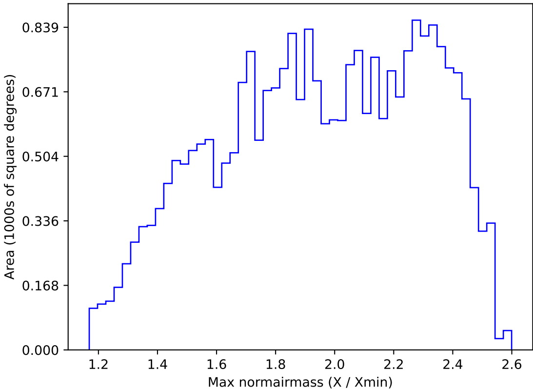
roll_pause_mjdp180_v3.4_10yrs All sky r band: Max normairmass
