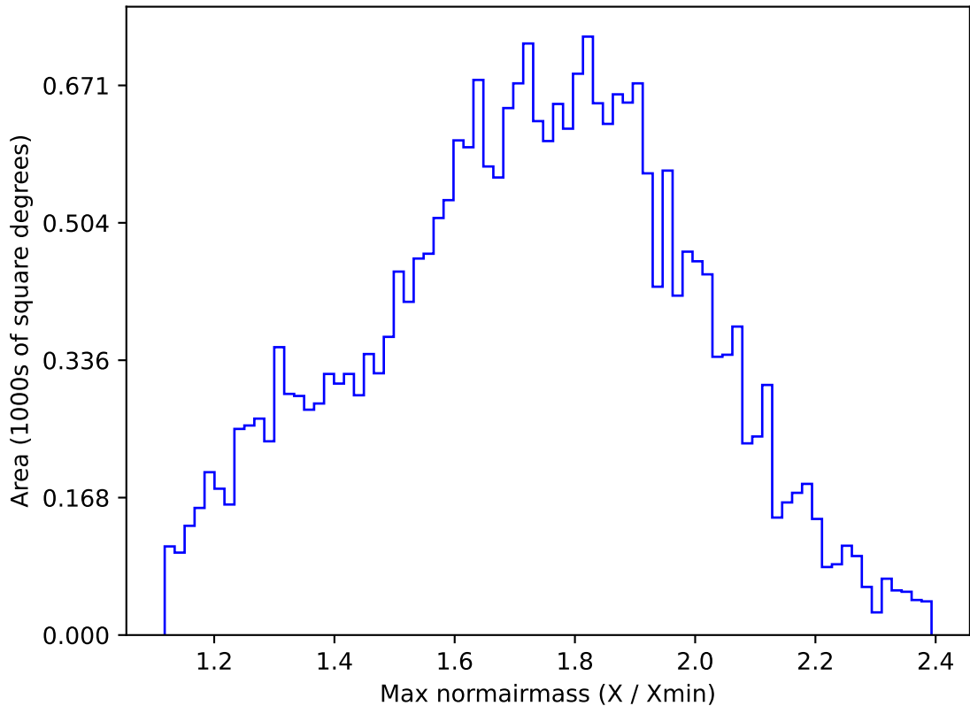
roll_pause_mjdp180_v3.4_10yrs All sky g band: Max normairmass
