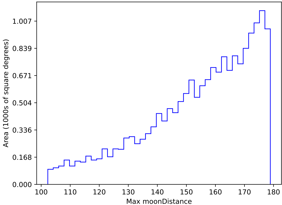
roll_pause_mjdp180_v3.4_10yrs WFD z band: Max moonDistance
