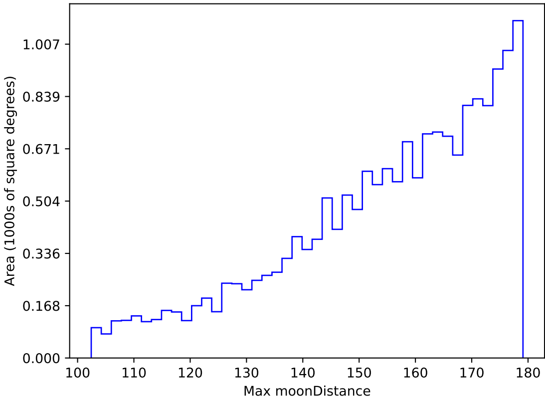
roll_pause_mjdp180_v3.4_10yrs WFD u band: Max moonDistance
