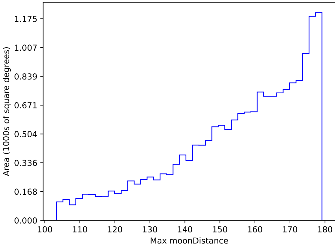
roll_pause_mjdp180_v3.4_10yrs WFD i band: Max moonDistance
