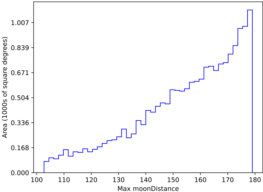
roll_pause_mjdp180_v3.4_10yrs WFD g band: Max moonDistance
