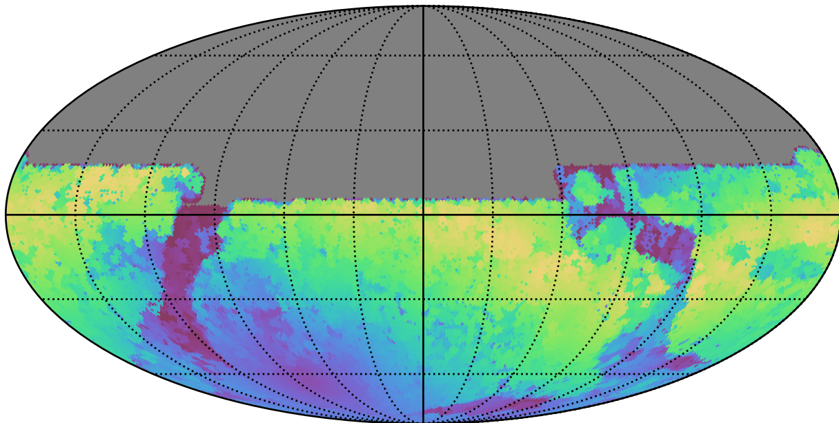
roll_pause_mjdp180_v3.4_10yrs All sky y band: Max moonDistance
