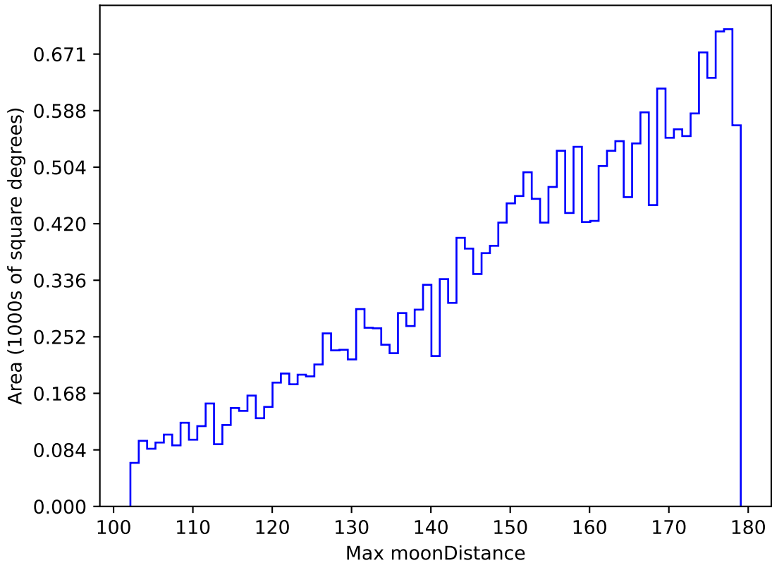
roll_pause_mjdp180_v3.4_10yrs All sky u band: Max moonDistance
