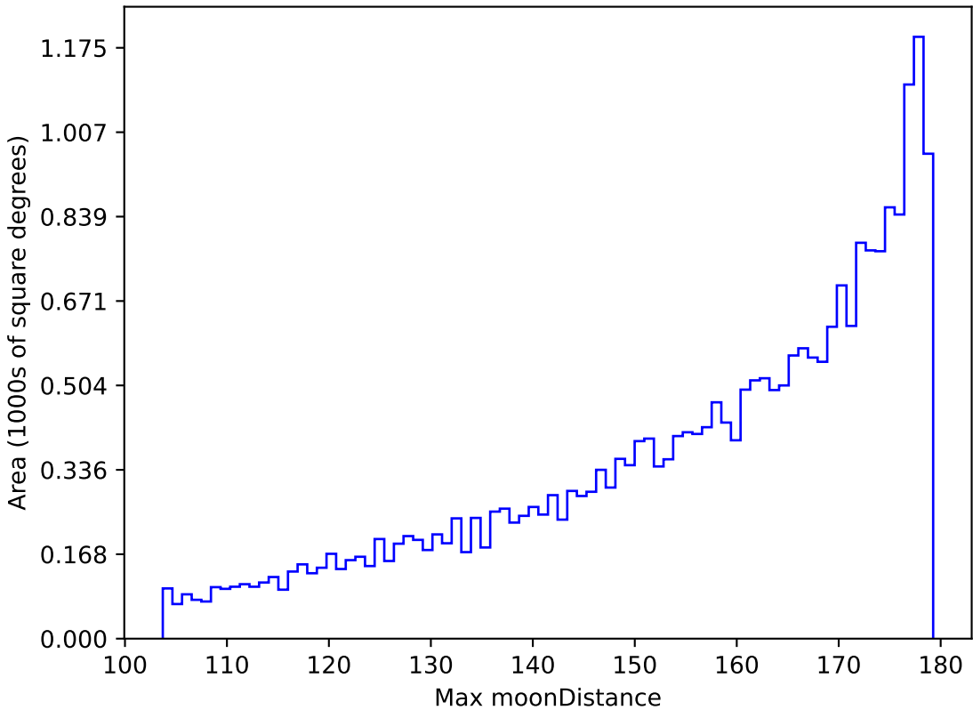
roll_pause_mjdp180_v3.4_10yrs All sky r band: Max moonDistance
