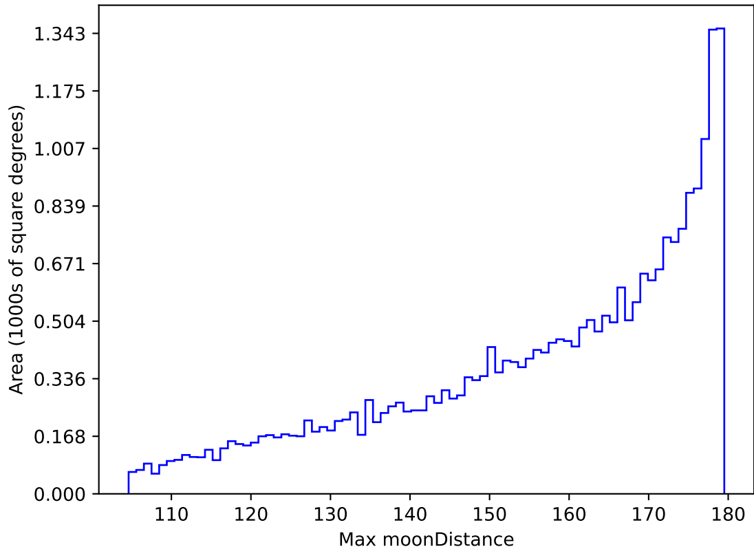
roll_pause_mjdp180_v3.4_10yrs All sky all bands: Max moonDistance
