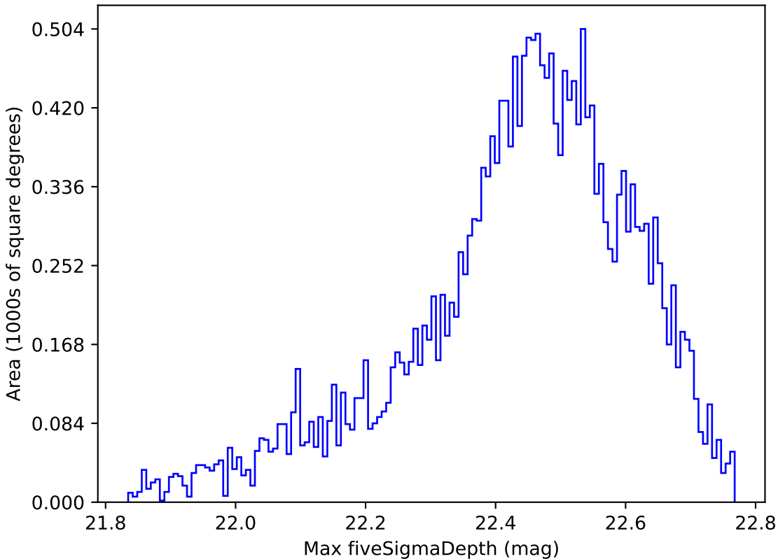
roll_pause_mjdp180_v3.4_10yrs Yr 1 y band: Max fiveSigmaDepth
