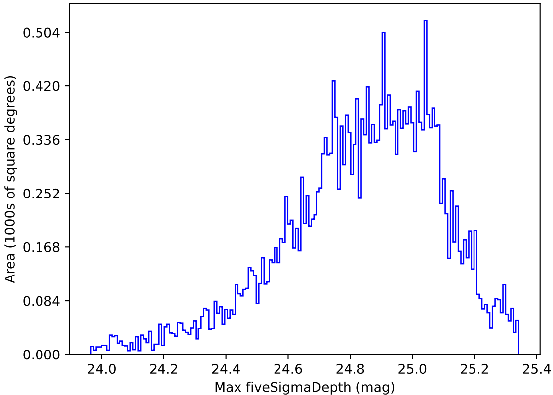
roll_pause_mjdp180_v3.4_10yrs Yr 1 g band: Max fiveSigmaDepth
