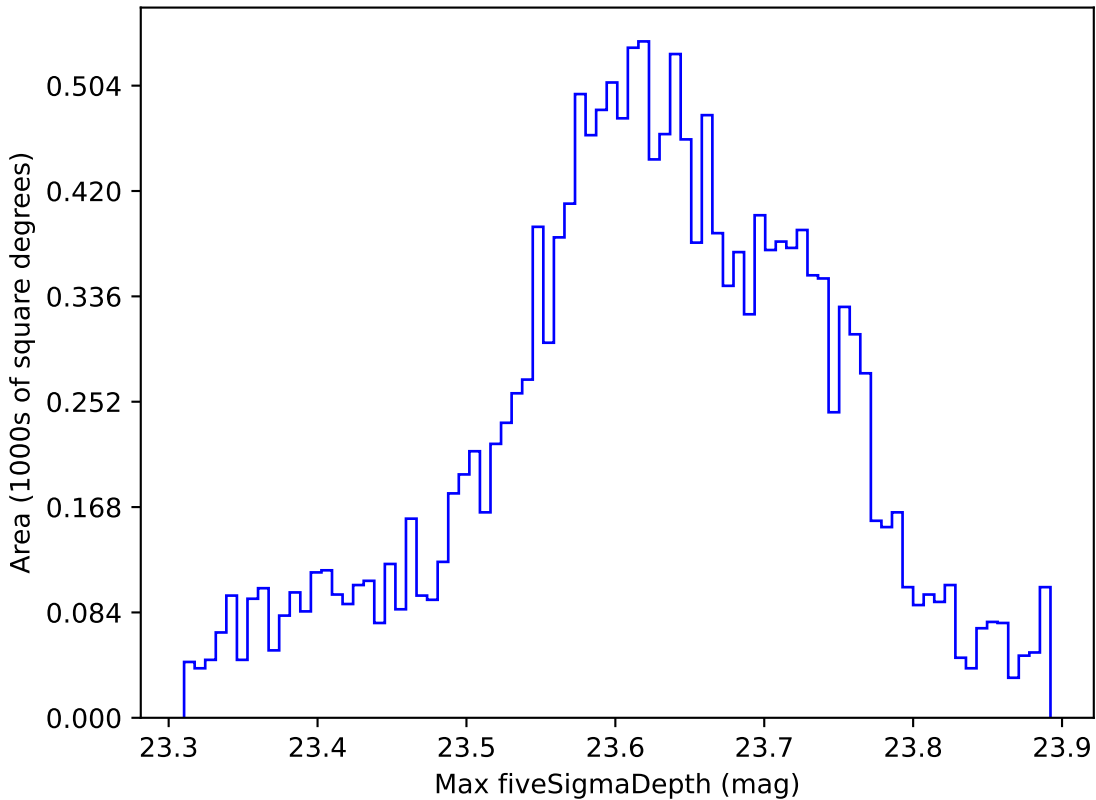
roll_pause_mjdp180_v3.4_10yrs WFD z band: Max fiveSigmaDepth
