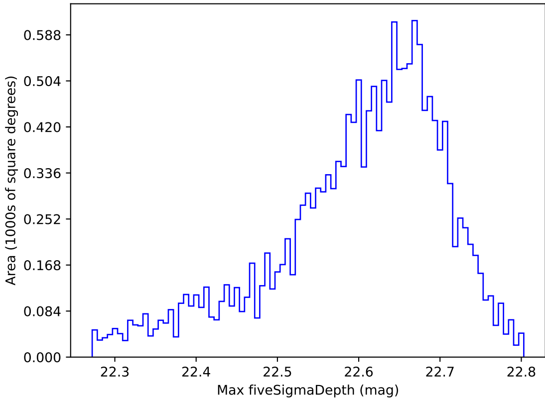
roll_pause_mjdp180_v3.4_10yrs WFD y band: Max fiveSigmaDepth
