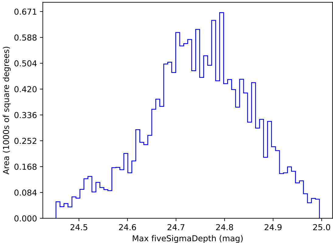
roll_pause_mjdp180_v3.4_10yrs WFD r band: Max fiveSigmaDepth
