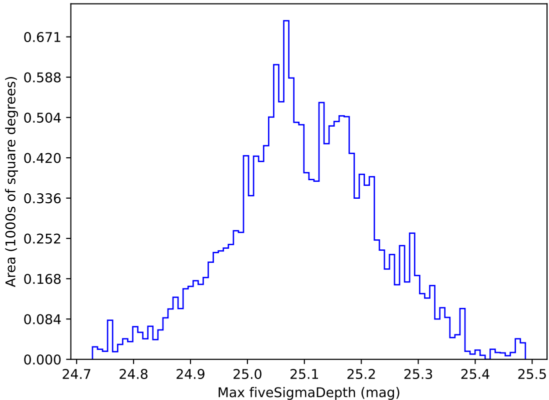
roll_pause_mjdp180_v3.4_10yrs WFD g band: Max fiveSigmaDepth
