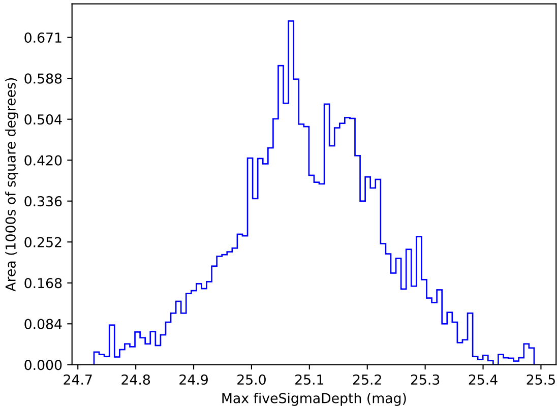
roll_pause_mjdp180_v3.4_10yrs WFD all bands: Max fiveSigmaDepth
