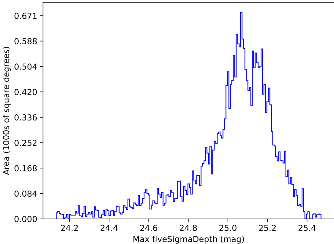
roll_pause_mjdp180_v3.4_10yrs All sky g band: Max fiveSigmaDepth
