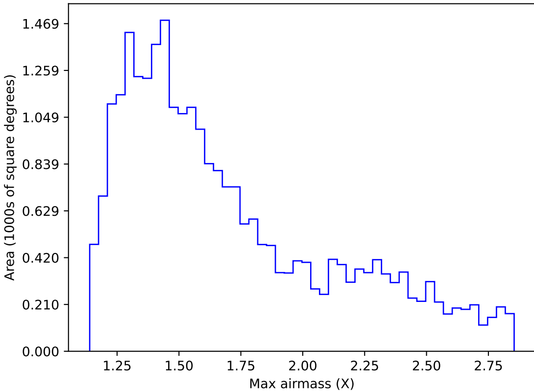
roll_pause_mjdp180_v3.4_10yrs Yr 1 i band: Max airmass
