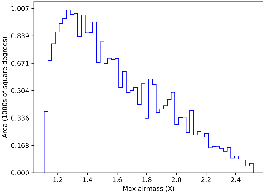
roll_pause_mjdp180_v3.4_10yrs Yr 1 g band: Max airmass
