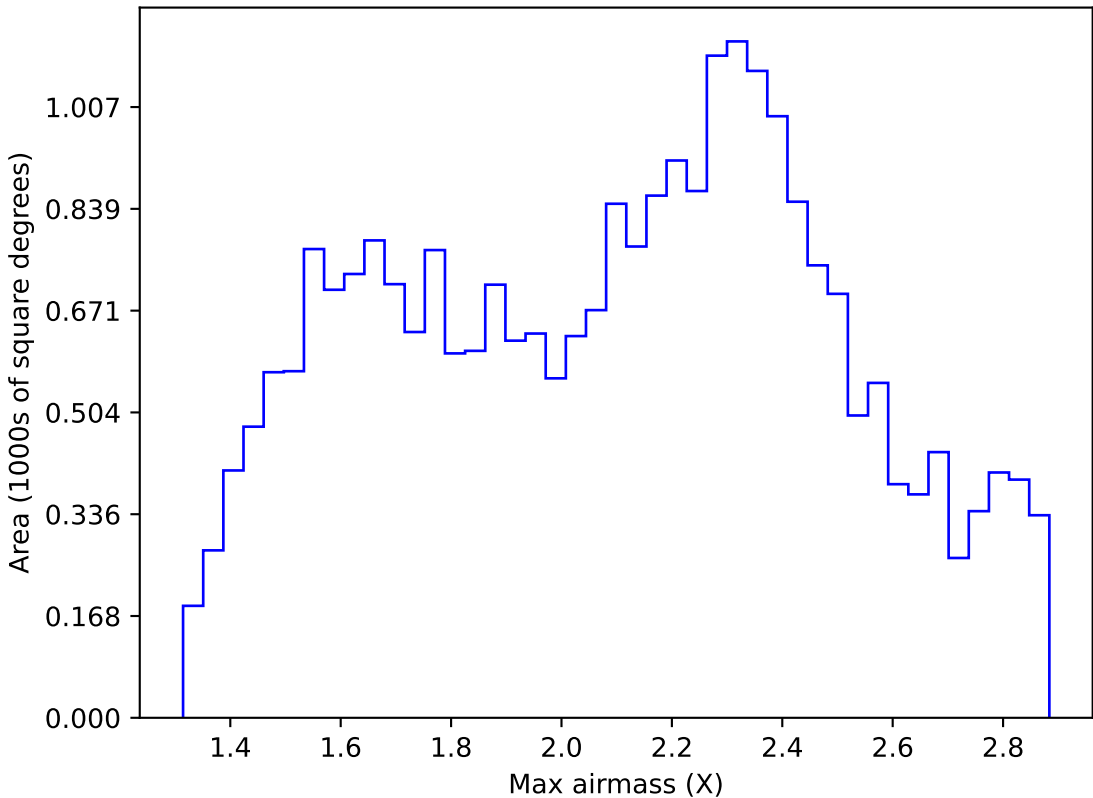
roll_pause_mjdp180_v3.4_10yrs Yr 1 all bands: Max airmass
