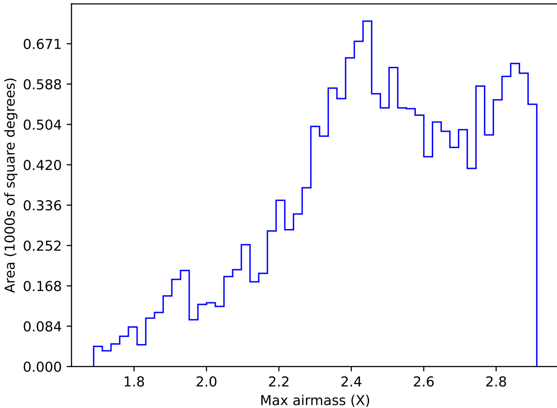
roll_pause_mjdp180_v3.4_10yrs WFD z band: Max airmass
