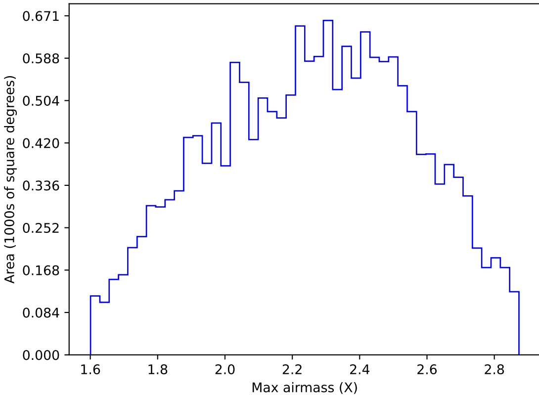
roll_pause_mjdp180_v3.4_10yrs WFD y band: Max airmass
