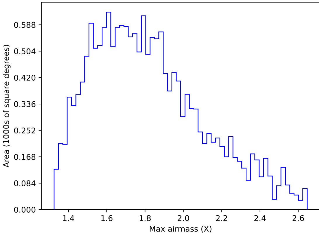
roll_pause_mjdp180_v3.4_10yrs WFD u band: Max airmass
