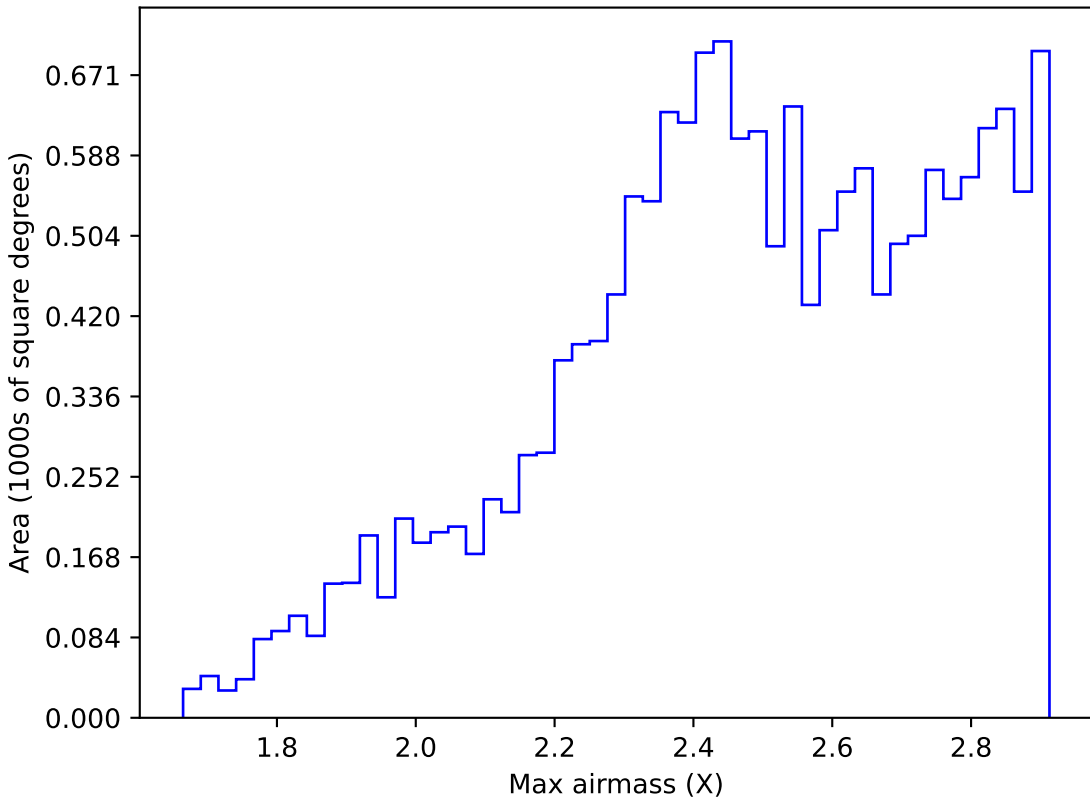
roll_pause_mjdp180_v3.4_10yrs WFD i band: Max airmass
