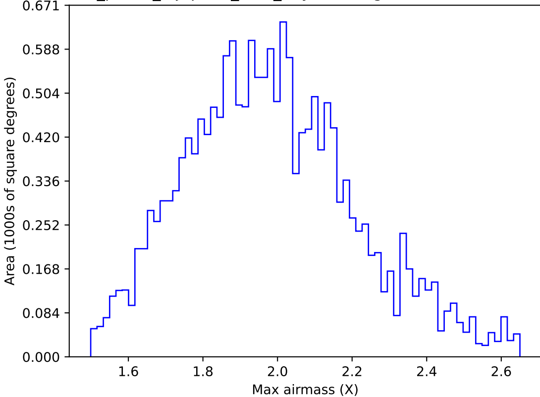
roll_pause_mjdp180_v3.4_10yrs WFD g band: Max airmass
