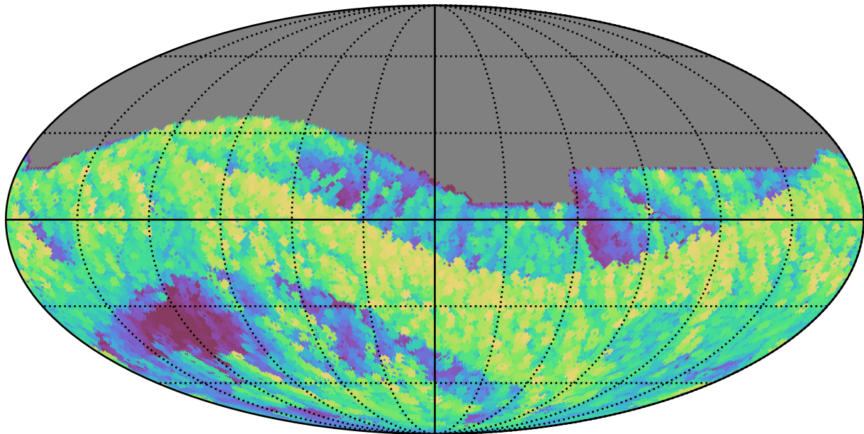
roll_pause_mjdp180_v3.4_10yrs All sky z band: Max airmass
