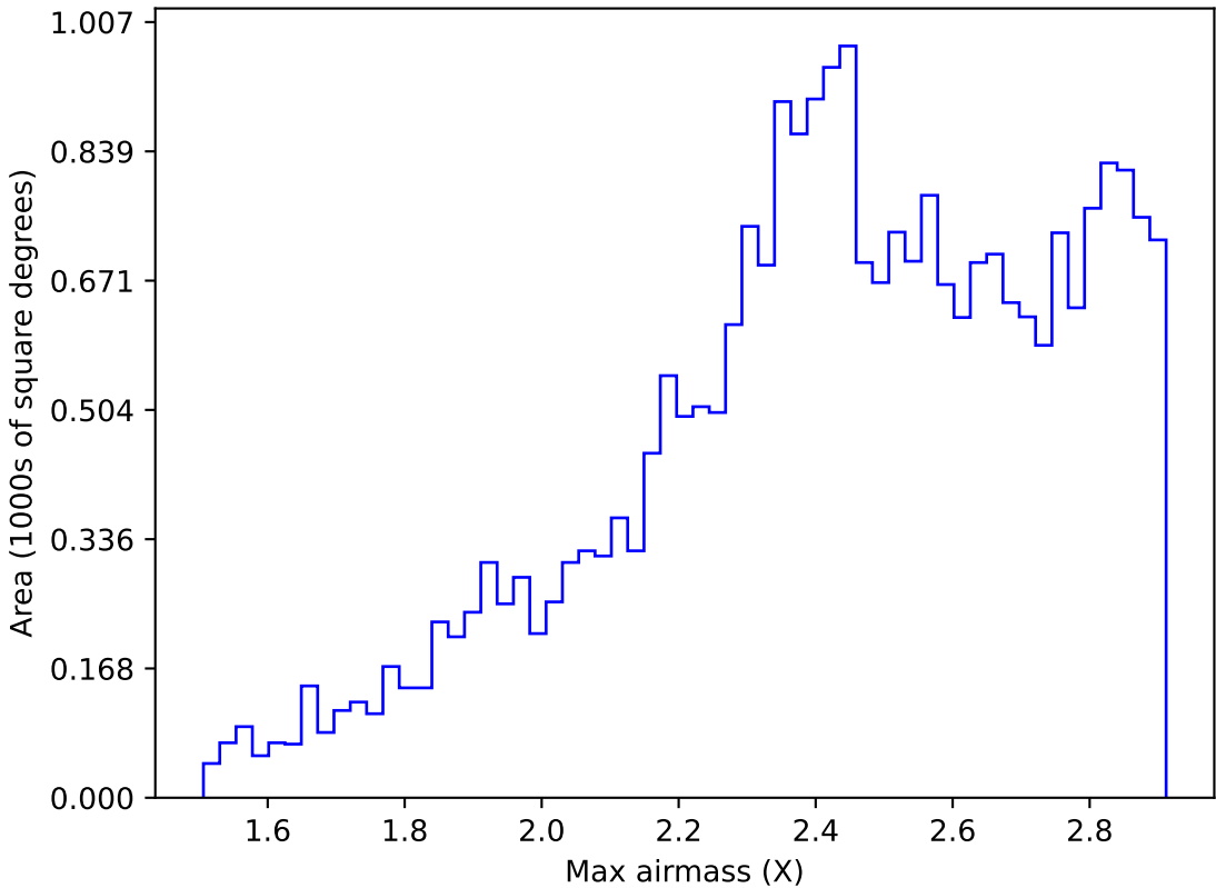
roll_pause_mjdp180_v3.4_10yrs All sky z band: Max airmass
