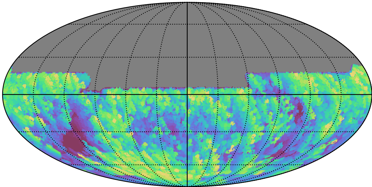
roll_pause_mjdp180_v3.4_10yrs All sky y band: Max airmass
