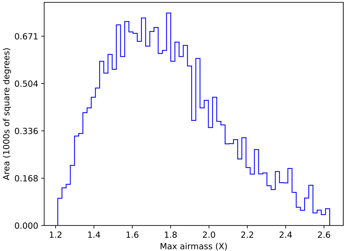
roll_pause_mjdp180_v3.4_10yrs All sky u band: Max airmass
