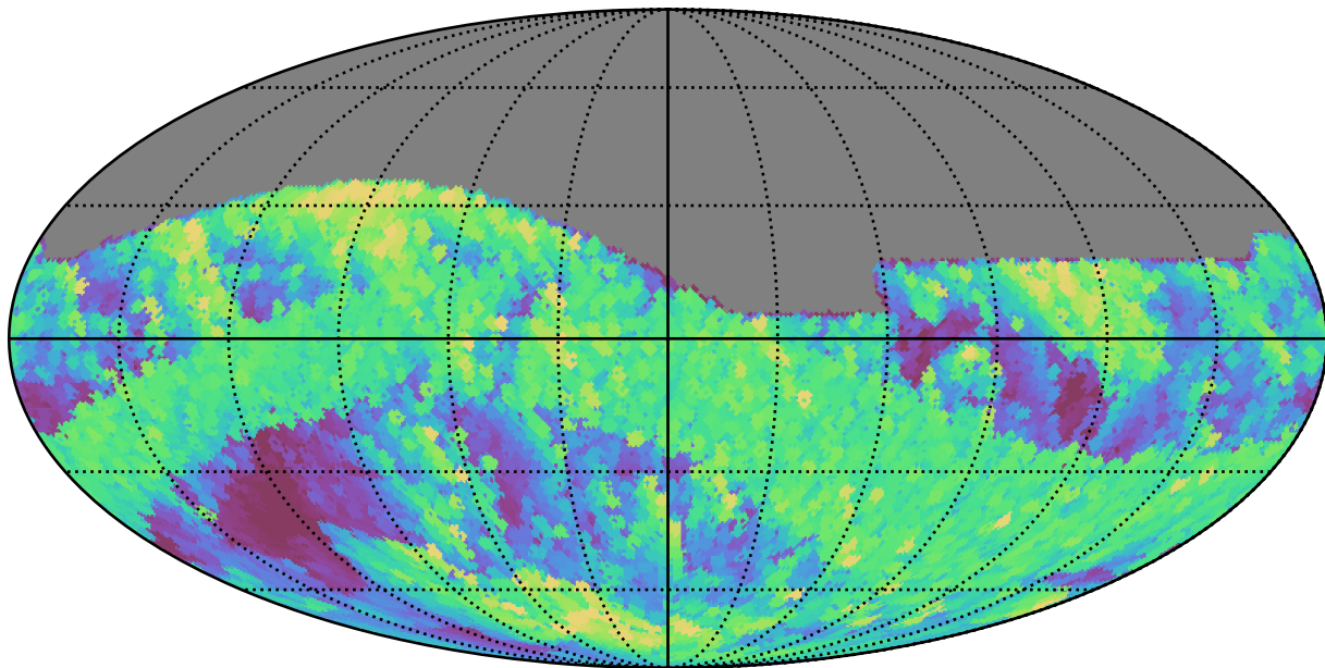
roll_pause_mjdp180_v3.4_10yrs All sky r band: Max airmass
