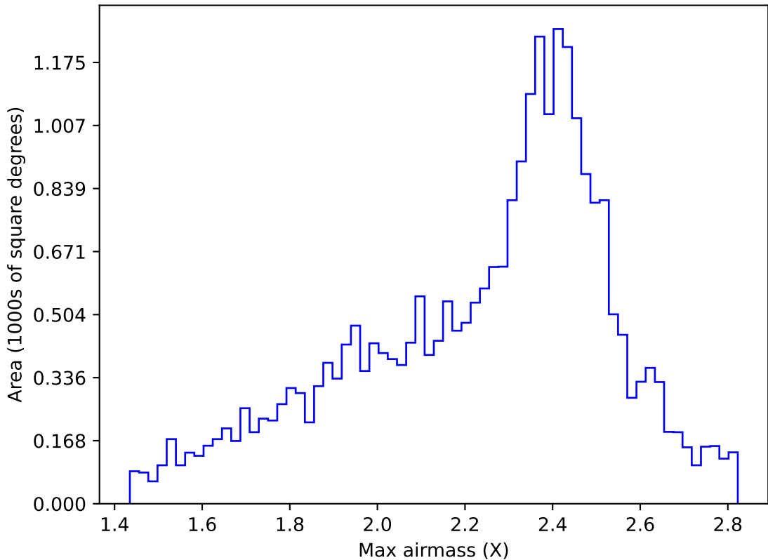
roll_pause_mjdp180_v3.4_10yrs All sky r band: Max airmass
