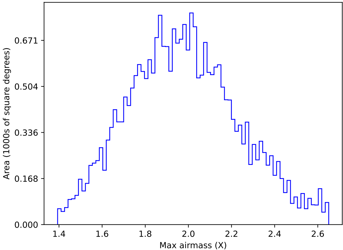
roll_pause_mjdp180_v3.4_10yrs All sky g band: Max airmass
